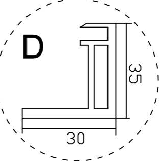
Frame cross-section
